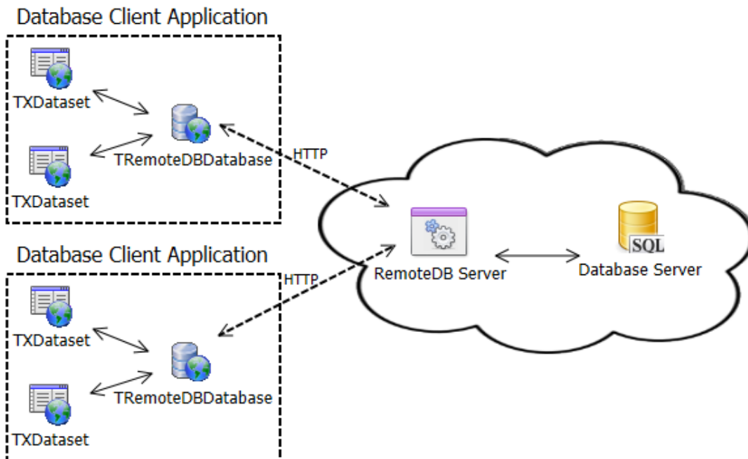
Overview of RemoteDB architecture.
